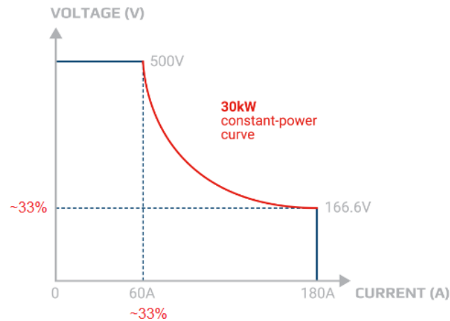
EA-PSI 10500-180
